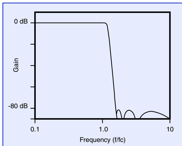
SR640 gain response
